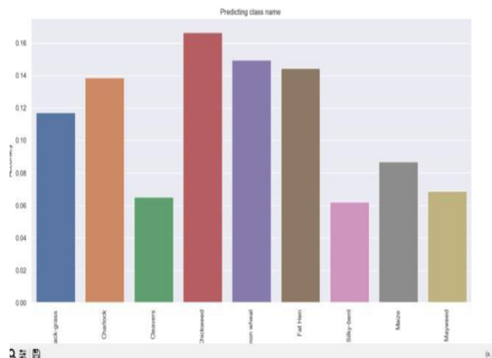
Fig. 4: Prediction Graph
