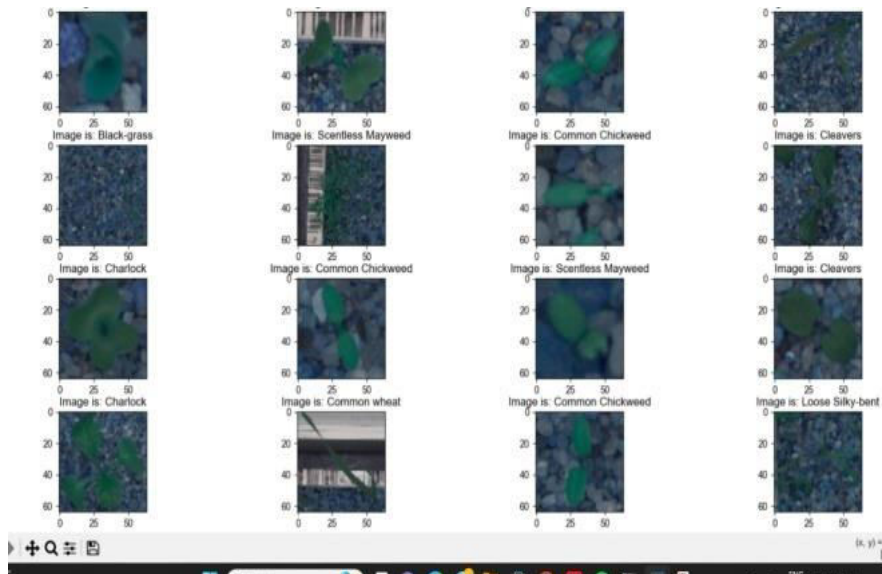
Fig. 6: Predicting Weed
