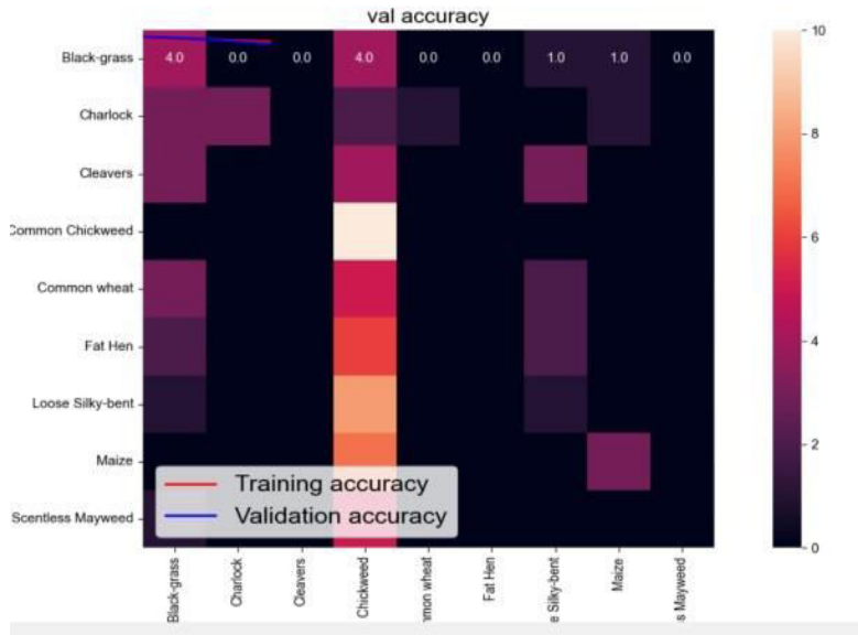
Fig. 5: Accuracy Graph
