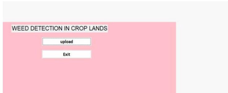
Fig. 2: Upload
