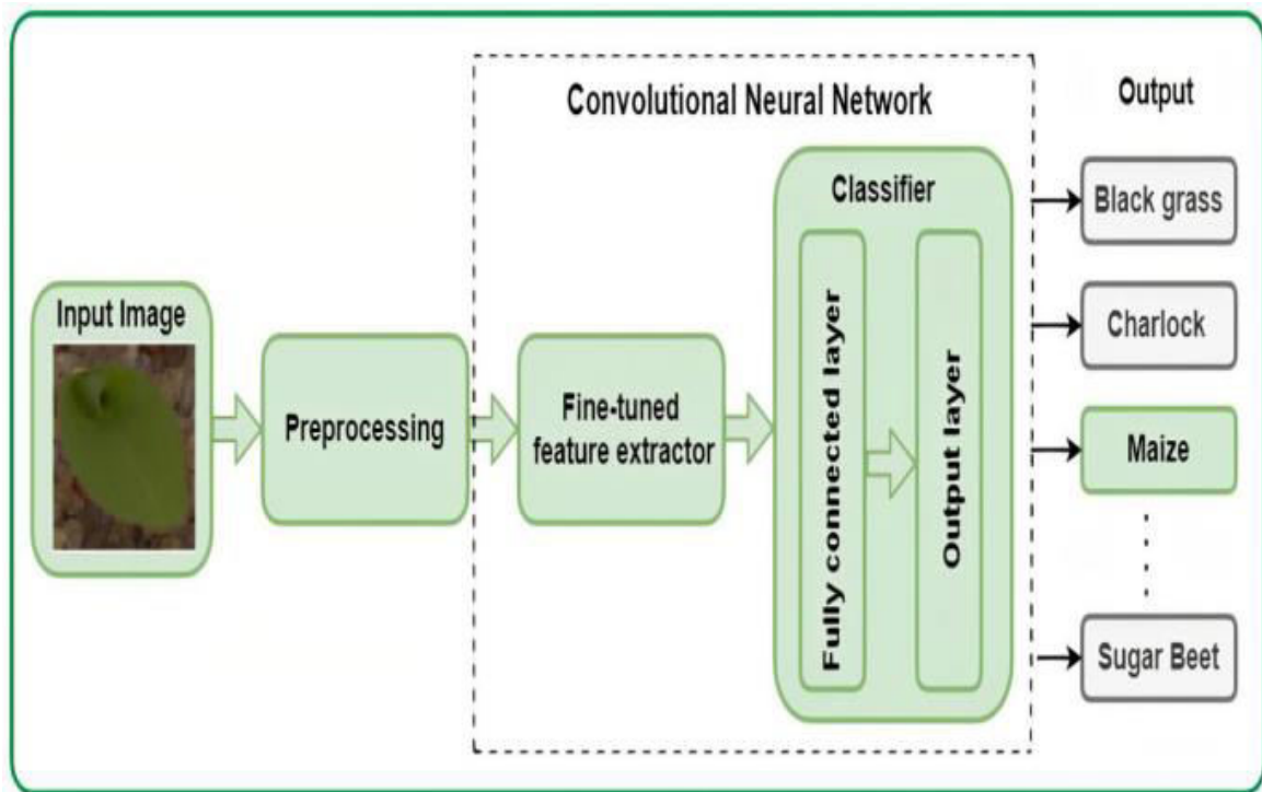
Fig. 1: System Overview
